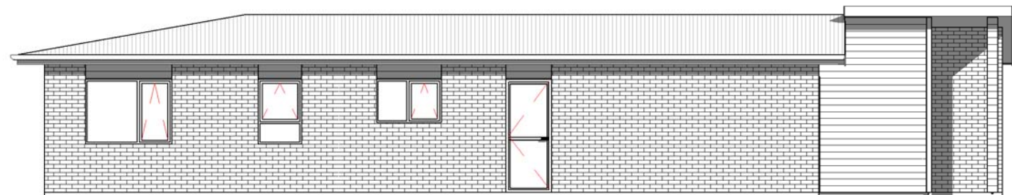
S South 1 : 100
